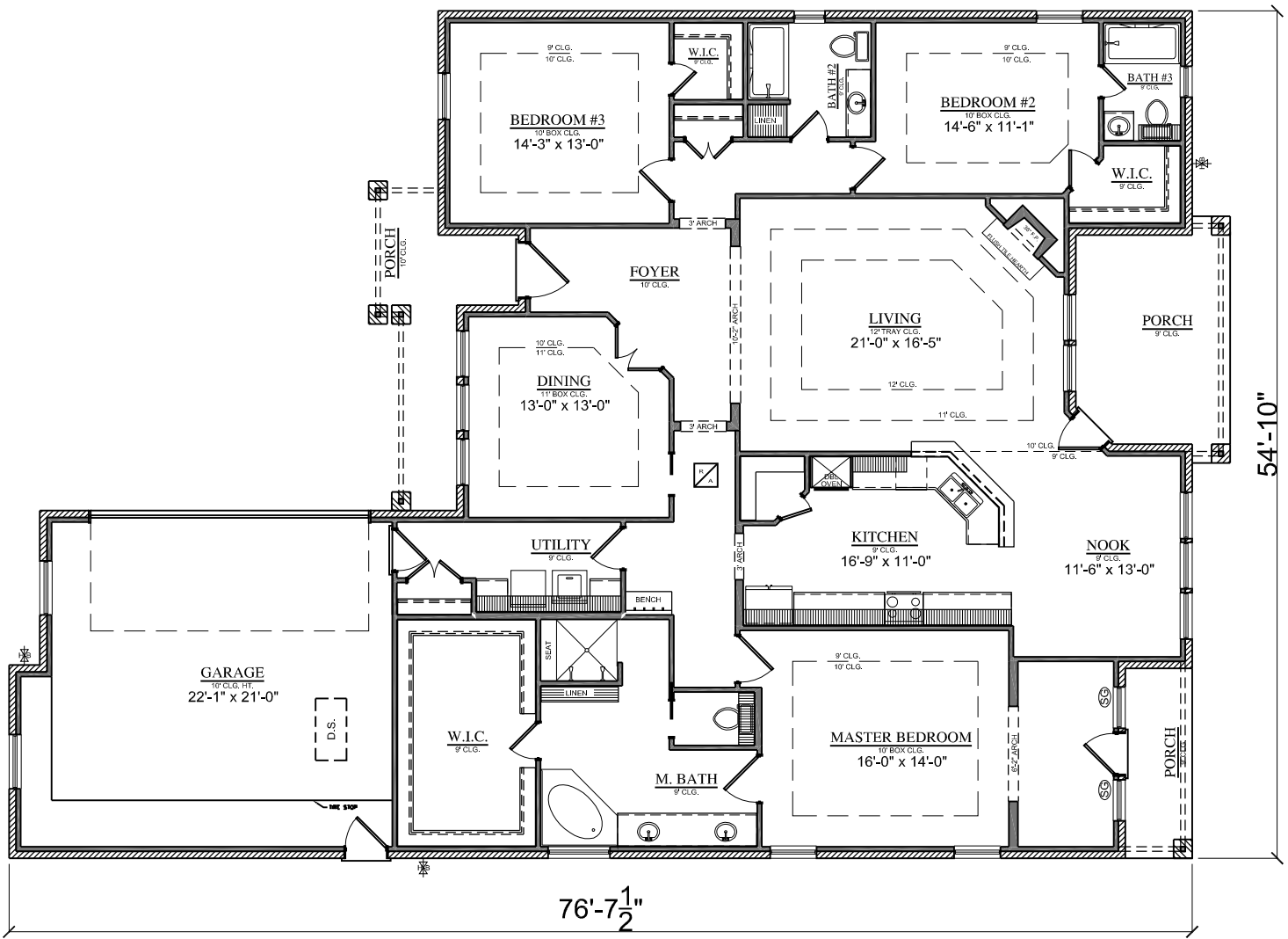
Floor Plan
